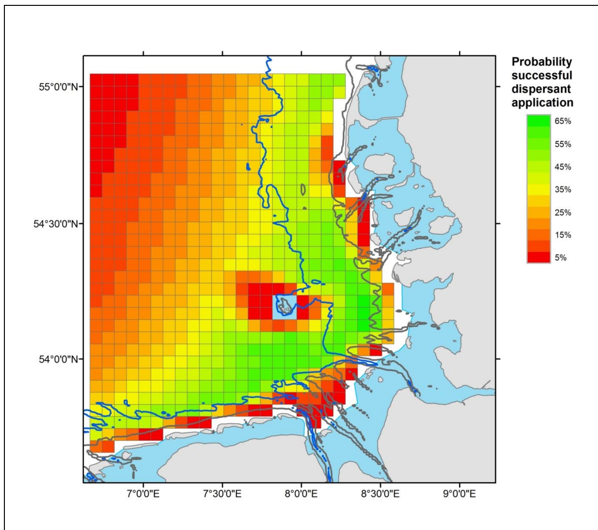
Figure 6.4: Probabilities that application of a 100% effective dispersant right after oil was released would reduce the amount of oil entering sensitive coastal areas by at least 95%. The grey (blue) line indicates the 10m (20m) depth line. The figure is reproduced from Schwichtenberg et al. (2016).
